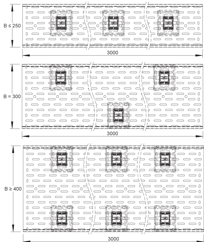
Number and arrangement of spacers AHG 62 when using different cable tray widths
